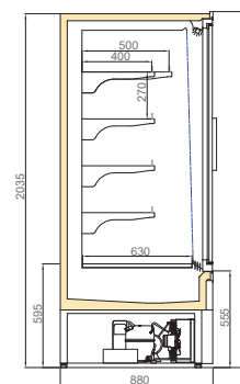
LISTER DGD/VWL 900/H2050
