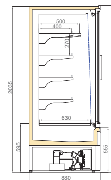
LISTER DGD/VNZ 900/H2050
